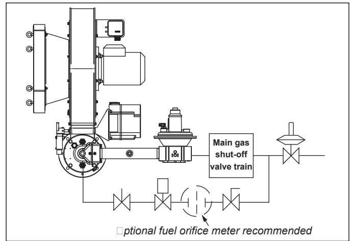
Figure 3.9. Pilot Start (Optional)
