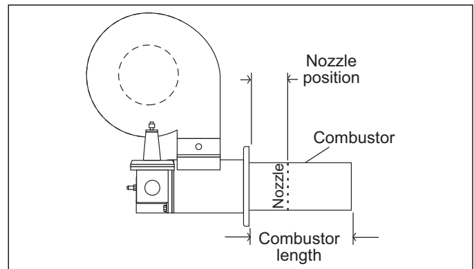
Figure 3.2. Combustor Length
