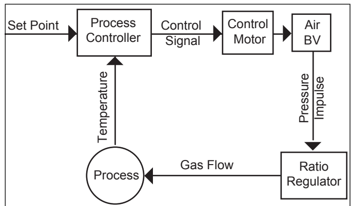
Figure 3.7. Basic Control Loop
