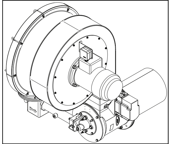
Figure 1.1. RatioMatic Burner (RM0050 - RM0700)
