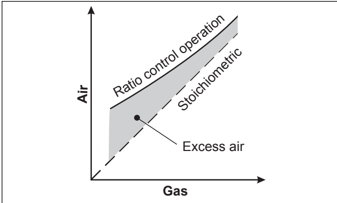
Figure 3.4. Air : Gas Flow
