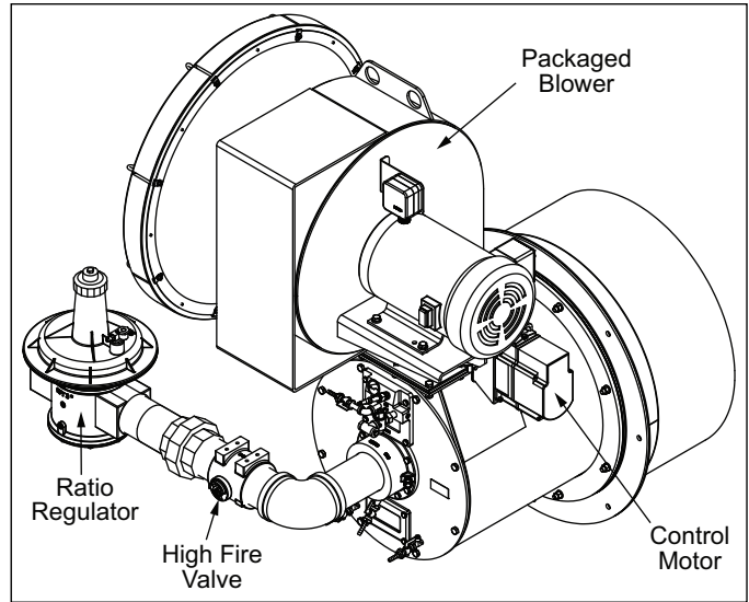
Figure 3.6. Basic Burner Component (RM1000 - RM3000)
