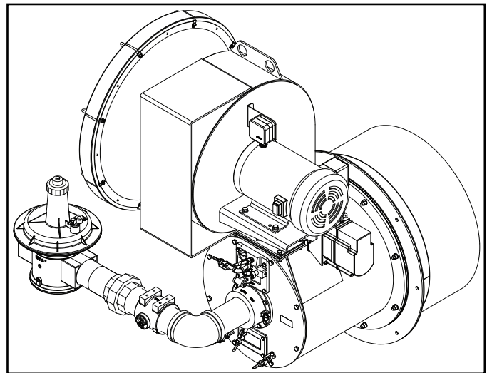
Figure 1.2. RatioMatic Burner (RM1000 - RM3000)
